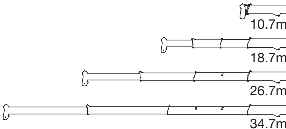
Boom Length
