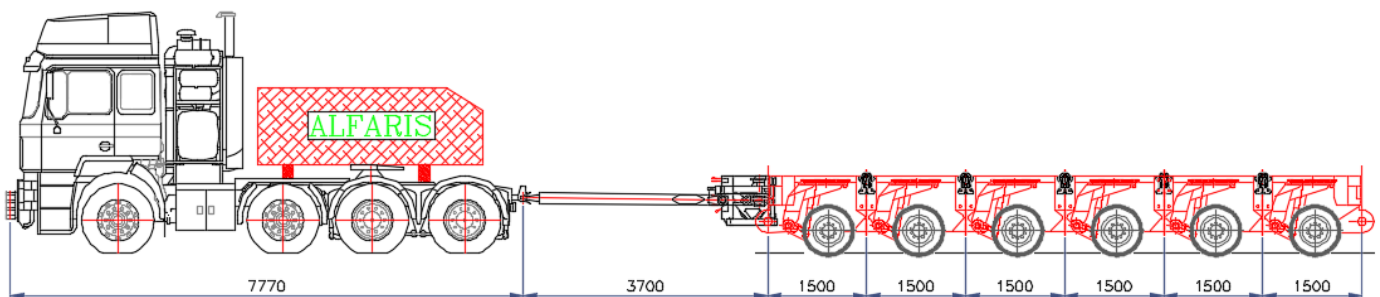
ELEVATION VIEW (MINIMUM AXLE LINE)
